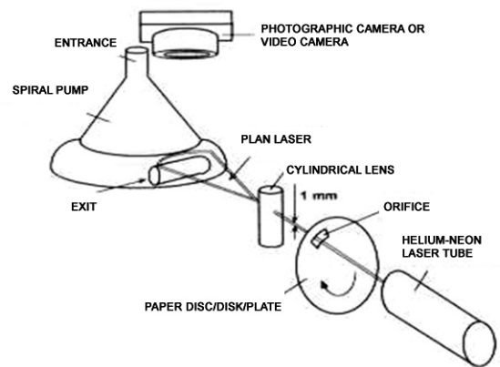
Fig. 4 – Visualization Flow Method with helium-neon planar laser
